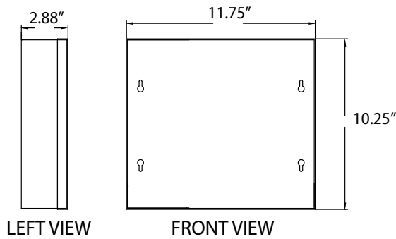
CORAYVAC® HEATING CONTROL [7.8 lbs.] [3.5 kg.]
